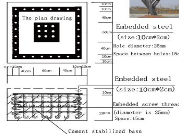
The working drawing for base of sculpture ( 5 m)
