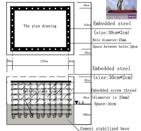
The working drawing for base of sculpture (10m)
