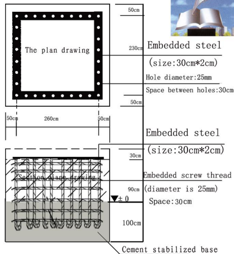
The working drawing for base of sculpture (10m)
