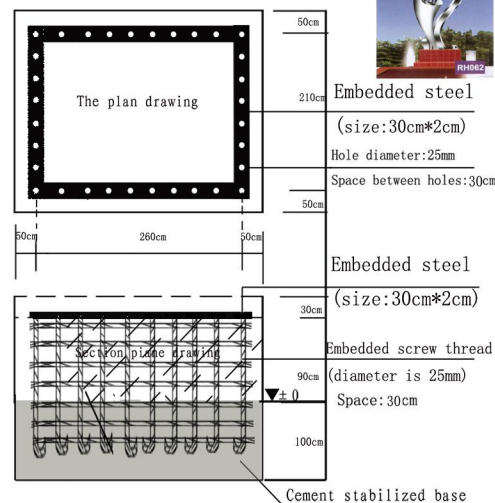
The working drawing for base of sculpture (10m)
